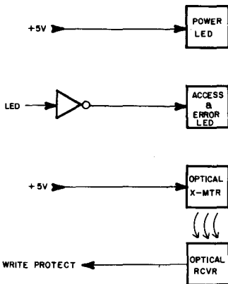
Fig. 7-43. Block diagram of optics circuit, Model 1541.
